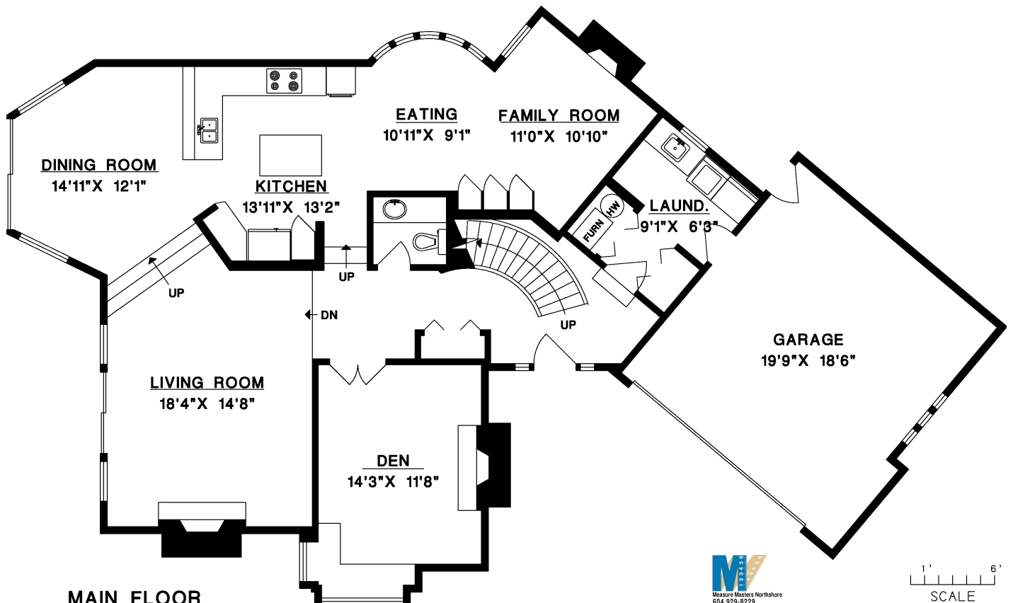
MAIN FLOOR
